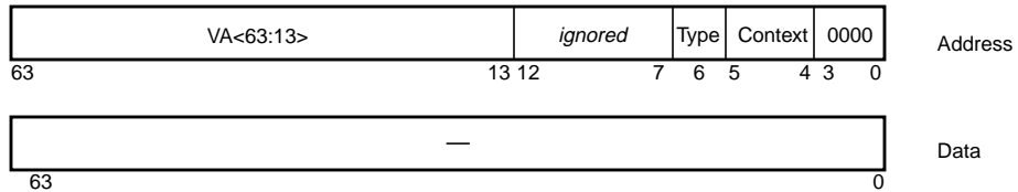
FIGURE 15-15 MMU Demap Operation Format
