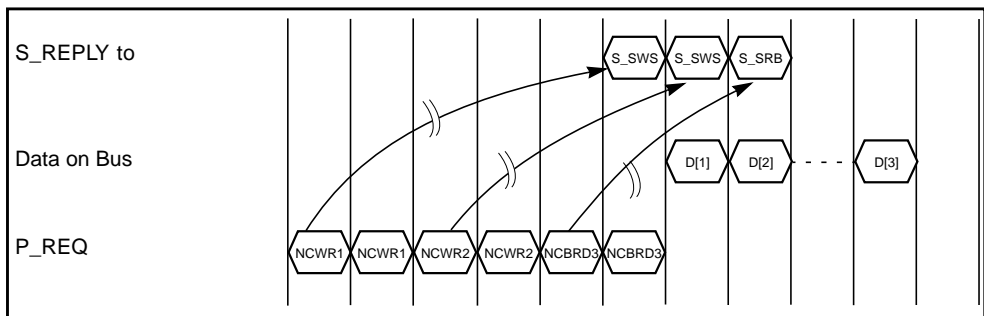
FIGURE E-5 S_REPLY Pipelining
