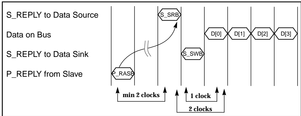
FIGURE E-4 P_REPLY to S_REPLY Timing
