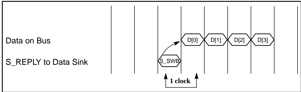
FIGURE E-3 S_REPLY Timing: UPA64S device Sinking Block
