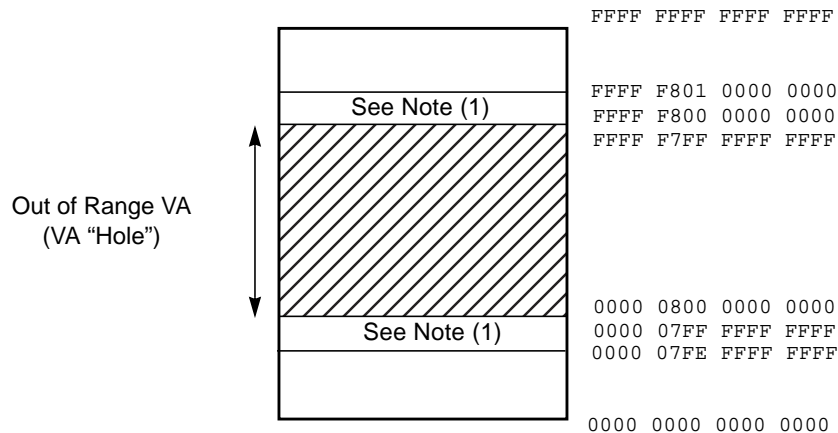
FIGURE 14-2 UltraSPARC-II i 's 44-bit Virtual Address Space, with Hole (Same as FIGURE 4-2 on page 25)
