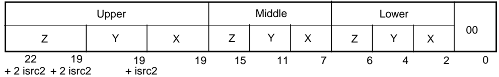
FIGURE 13-30 Three Dimensional Array Blocked-Address Format (Array32)
