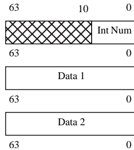
FIGURE 11-1 Mondo Vector Format
