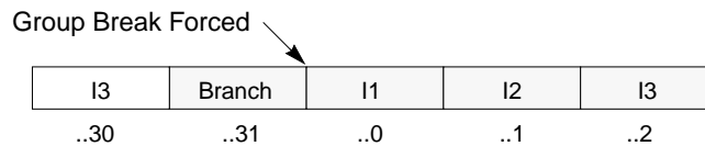
FIGURE 21-5 Artificial Branch Inserted after a 32-byte Boundary
