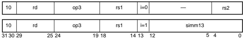
FIGURE 13-3 WRASR Format
