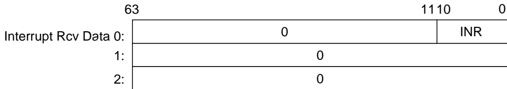
FIGURE 19-1 Interrupt Vector Data Registers Contents
