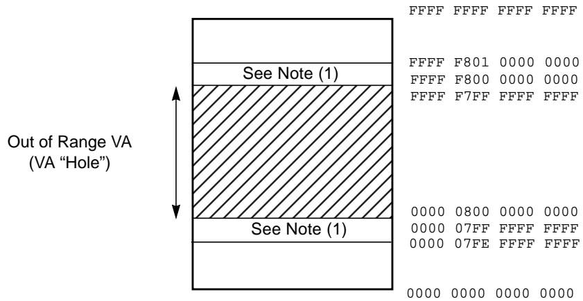
FIGURE 4-2 UltraSPARC-III 44-bit Virtual Address Space, with Hole (Same as FIGURE 14-2 on page 184)
