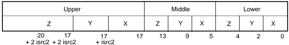
FIGURE 13-28 Three Dimensional Array Blocked-Address Format (Array8)
