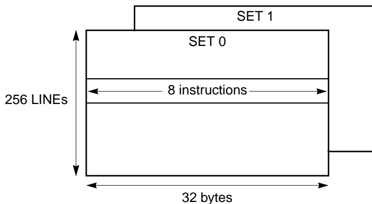
FIGURE 21-1 I-cache Organization
