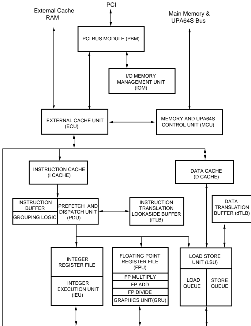
FIGURE 1-1 UltraSPARC-IIi Block Diagram
