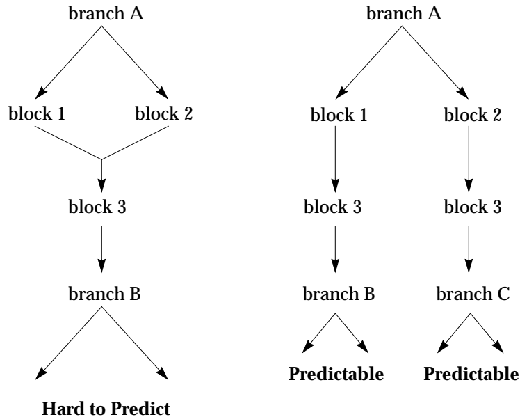
FIGURE 21-10 Branch Transformation to Reduce Mispredicted Branches
