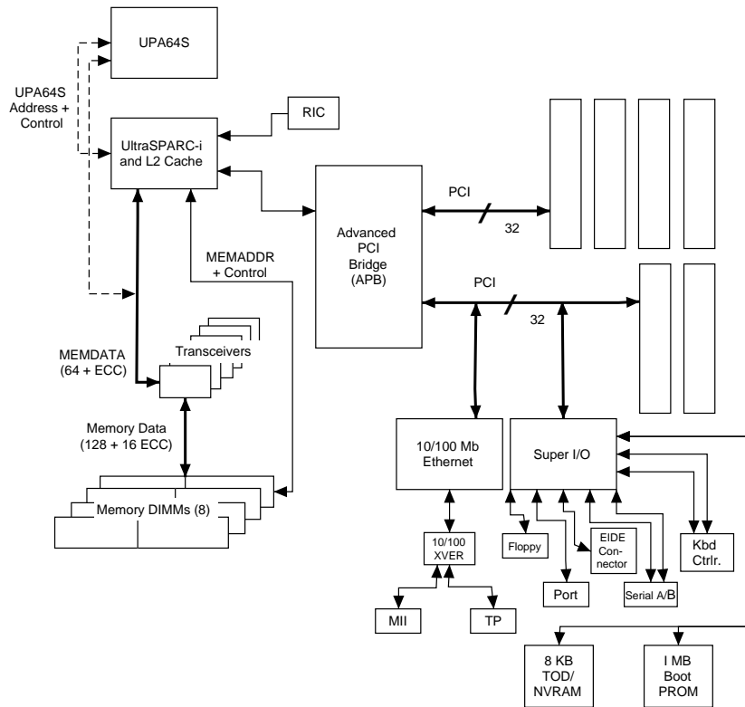
FIGURE 5-1 Overview of UltraSPARC-IIi Reference Platform
