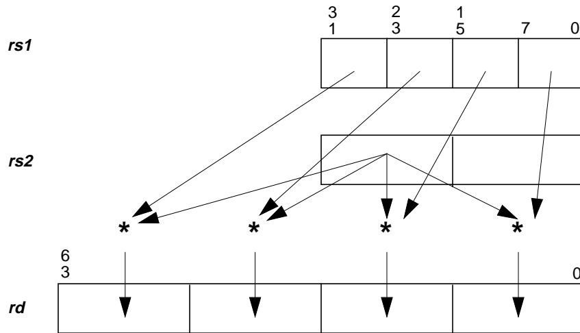
FIGURE 13-15 FMUL8x16AU Operation
