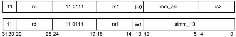
FIGURE 13-33 Format (3) STDA:
