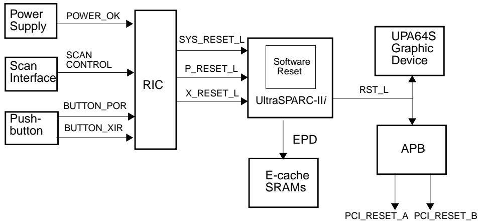
FIGURE 17-1 Reset Block Diagram
