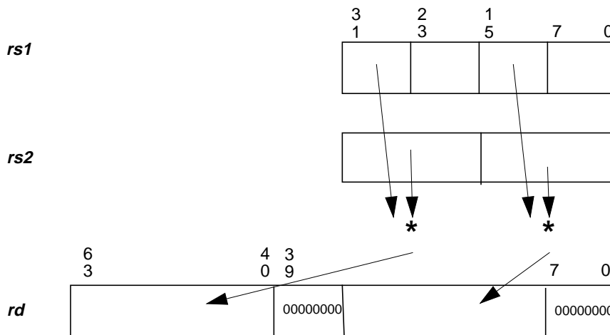
FIGURE 13-19 FMULD8SUx16 Operation
