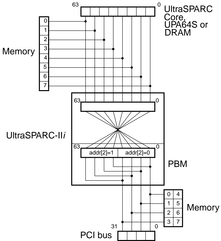
FIGURE 9-1 UltraSPARC-IIi Byte Twisting
