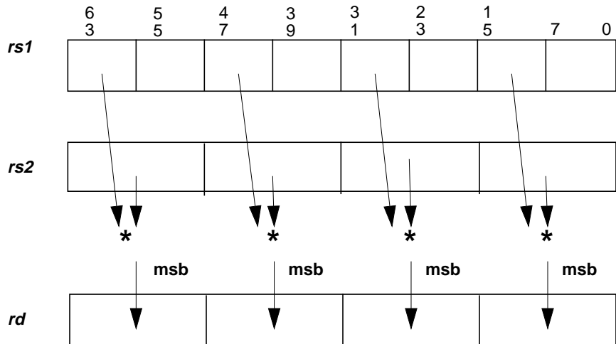
FIGURE 13-17 FMUL8SUx16 Operation
