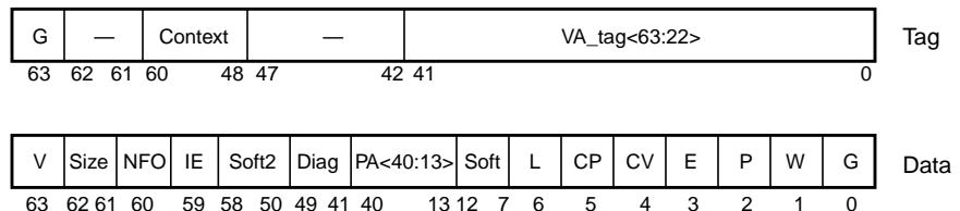
FIGURE 15-1 Translation Table Entry (TTE) (from TSB)
