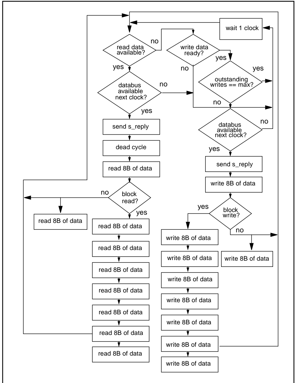
FIGURE E-8 UPA64s Transactions Flowchart—Data Bus
