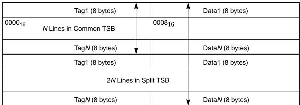
FIGURE 15-2 TSB Organization
