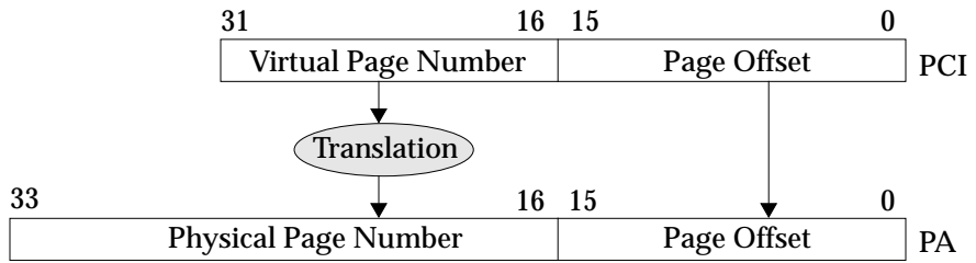
FIGURE 10-5 Virtual to Physical Address Translation for 64K Page Size
