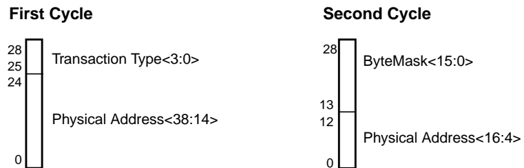
FIGURE E-6 Packet Format: Noncached P_REQ Transactions
