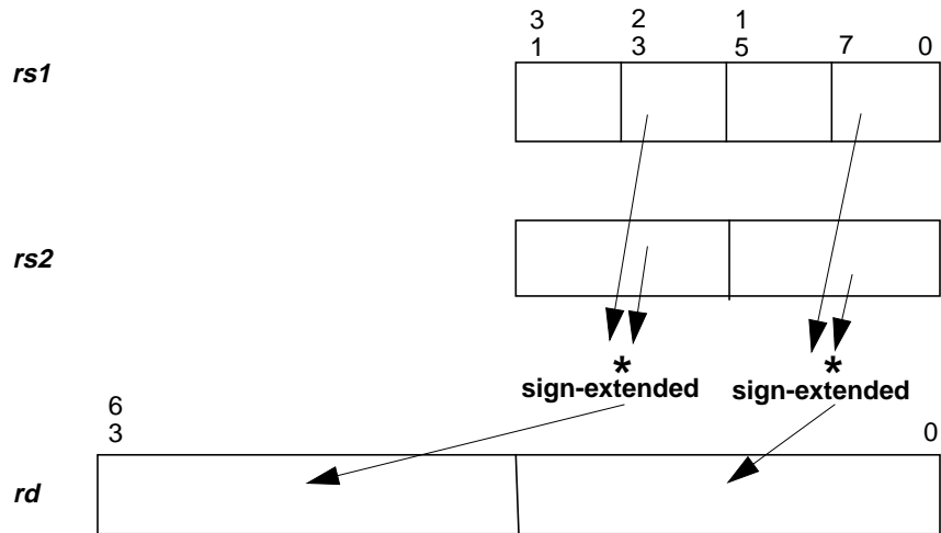
FIGURE 13-20 FMULD8ULx16 Operation
