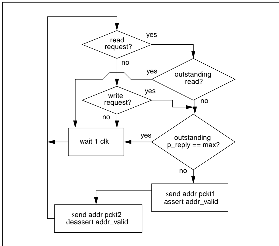
FIGURE E-7 UPA64s Transactions Flowchart—Address Bus
