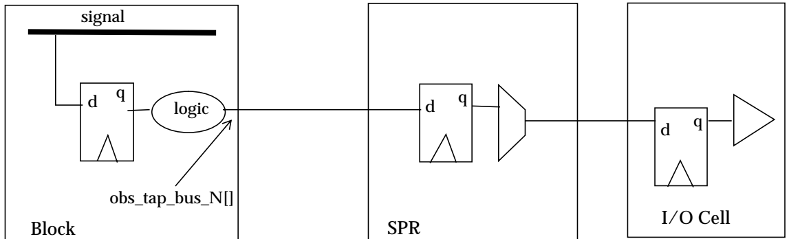
FIGURE I-2 Diagram of Observability Bus Logic.
