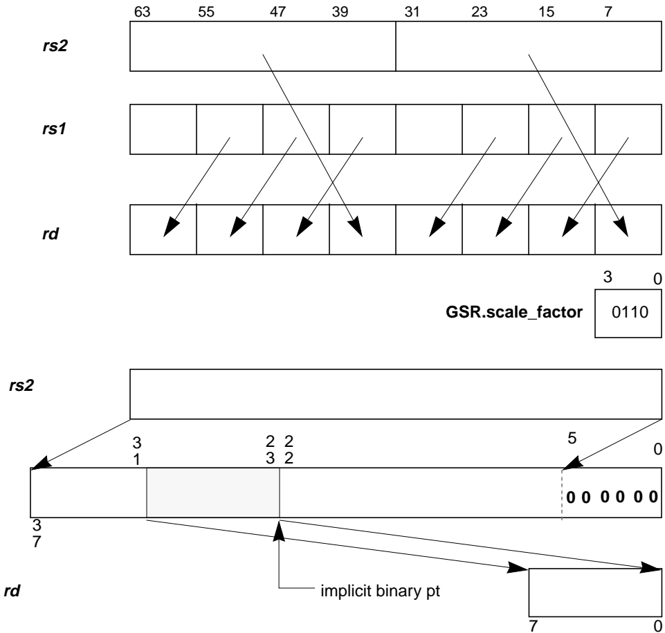
FIGURE 13-9 FPACK32 Operation
