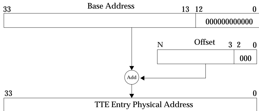
FIGURE 10-8 Computation of TTE Entry Address
