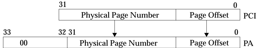
FIGURE 10-7 Physical Address Formation in Pass-through Mode (8K and 64K)
