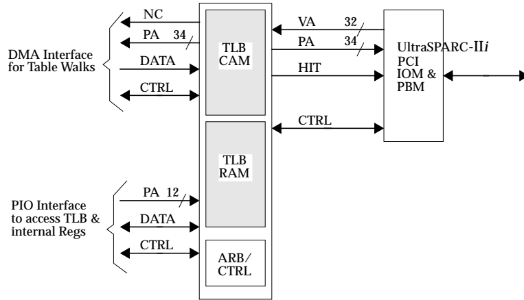
FIGURE 10-1 IOM Top Level Block Diagram
