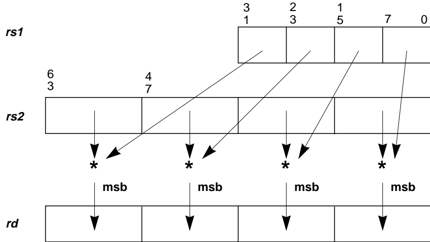
FIGURE 13-14 FMUL8x16 Operation
