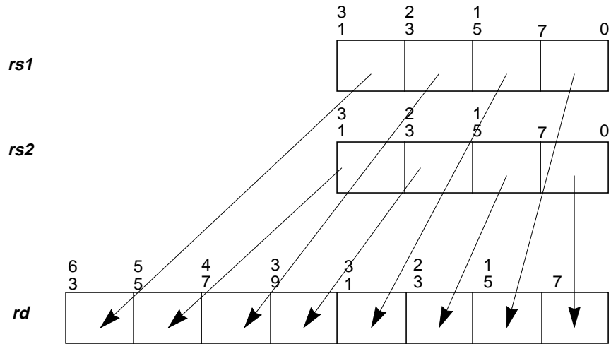
FIGURE 13-12 FPMERGE Operation
