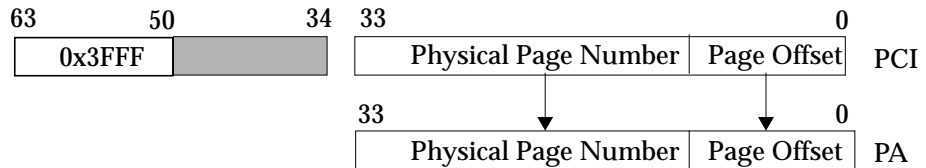
FIGURE 10-6 Physical Address Formation in Bypass Mode (8K and 64K)
