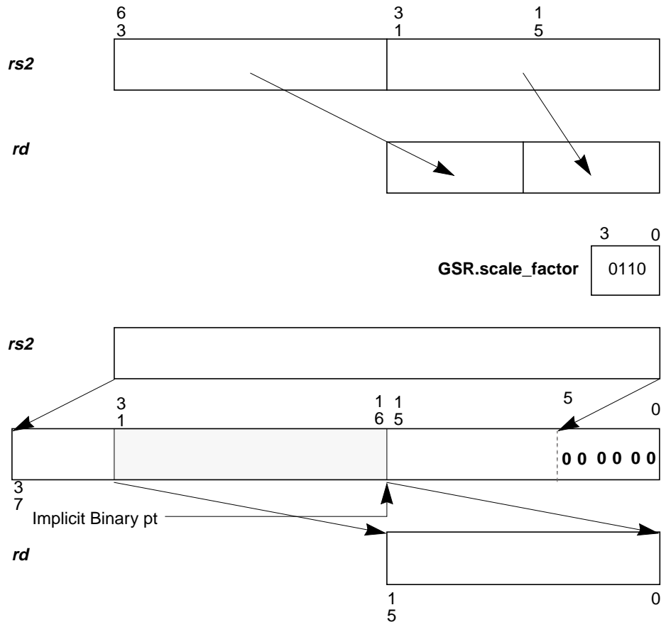
FIGURE 13-10 FPACKFIX Operation
