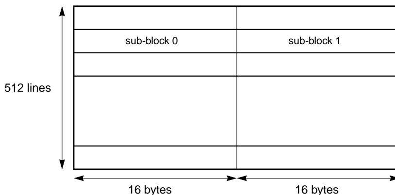
FIGURE 21-11 Logical Organization of D-cache
