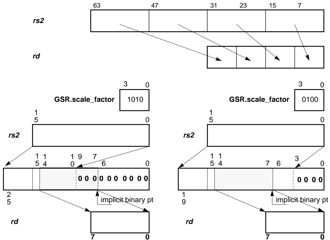
FIGURE 13-8 FPACK16 Operation
