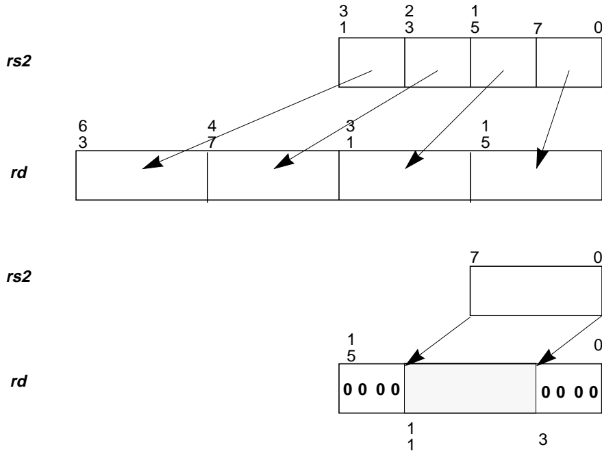
FIGURE 13-11 FEXPAND Operation
