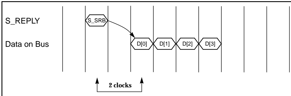
FIGURE E-2 S_REPLY Timing: UPA64S device Sourcing Block
