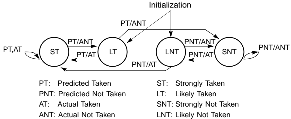
FIGURE 21-6 Dynamic Branch Prediction State Diagram
