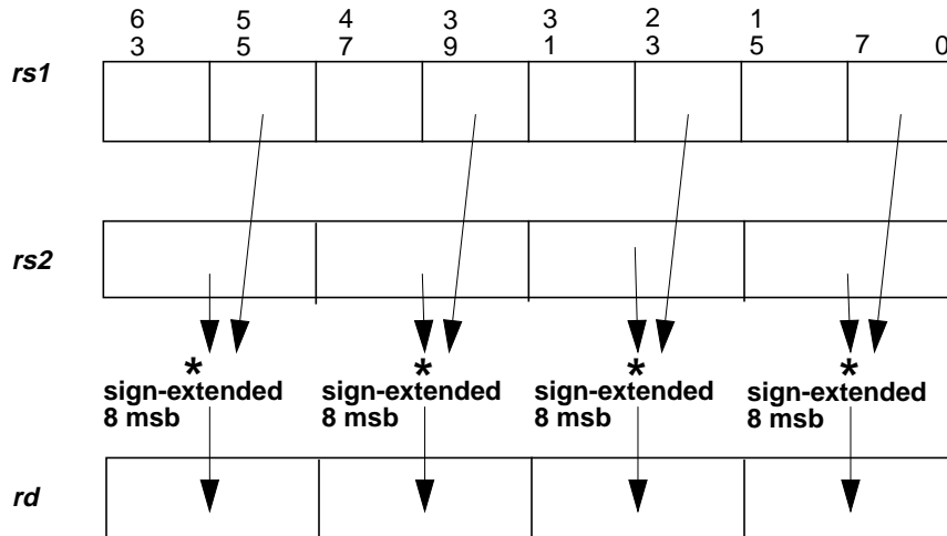
FIGURE 13-18 FMUL8ULx16 Operation
