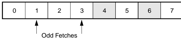
FIGURE 21-2 Odd Fetch to an I-cache Line
