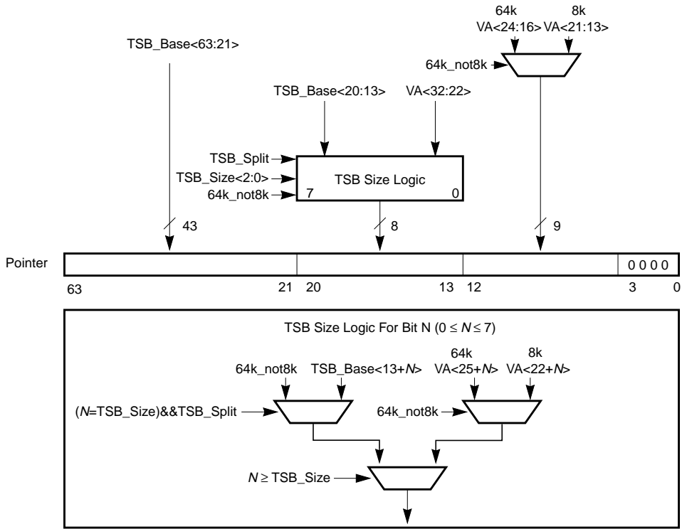
FIGURE 15-16 Formation of TSB Pointers for 8 kB and 64 kB TTEs
