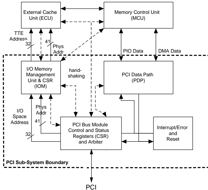
FIGURE 1-2 UltraSPARC-II i PCI and MCU Subsystems
