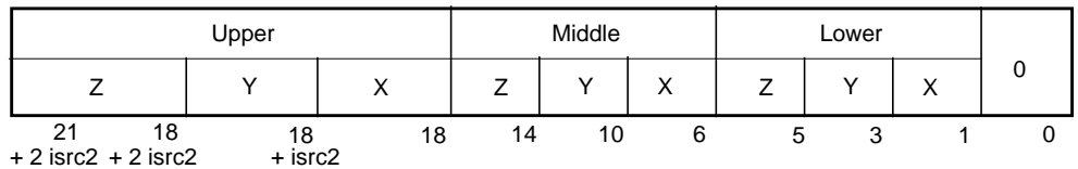
FIGURE 13-29 Three Dimensional Array Blocked-Address Format (Array16)
