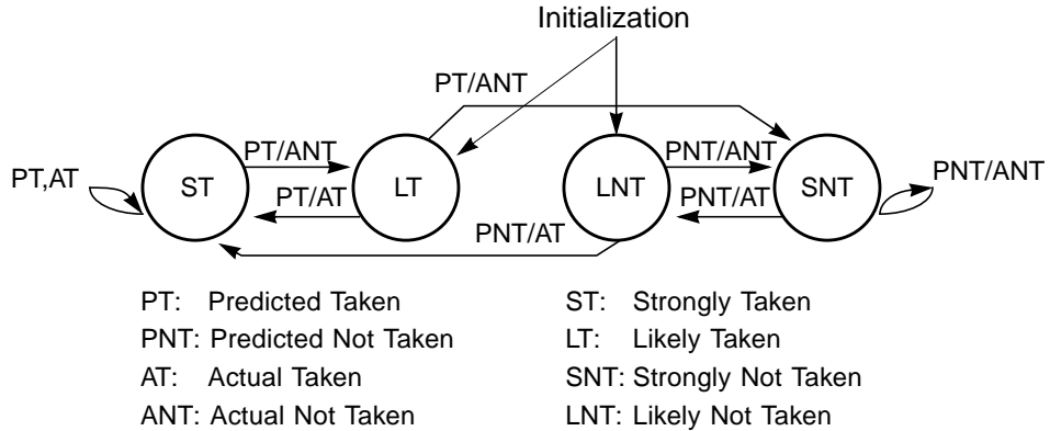
FIGURE A-14 Dynamic Branch Prediction State Diagram
