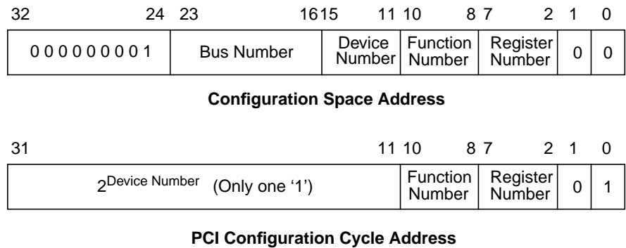
FIGURE 19-2 Type 0 Configuration Address Mapping
