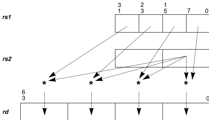
FIGURE 13-16 FMUL8x16AL Operation
