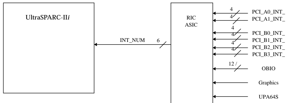
FIGURE 11-4 Interrupt Concentrator
