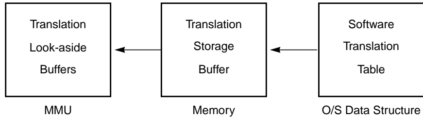
FIGURE 4-3 Software View of the UltraSPARC-IIi MMU
