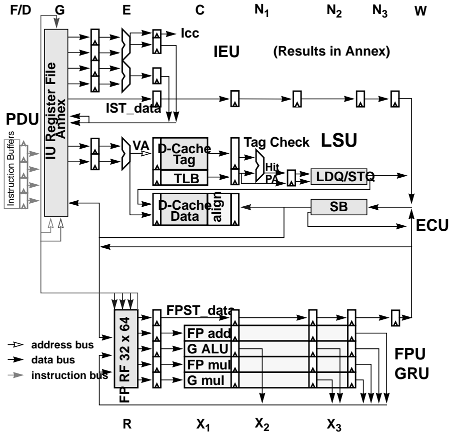
FIGURE 2-2 UltraSPARC-IIi Pipeline Stages (Detail)
