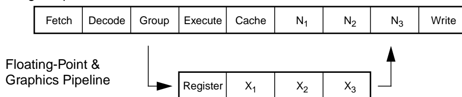
FIGURE 2-1 UltraSPARC-IIi Pipeline Stages (Simplified)
