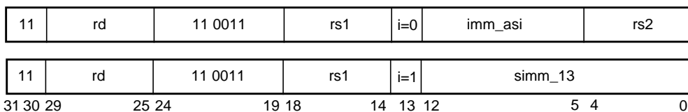
FIGURE 13-32 Format (3) LDDFA:
