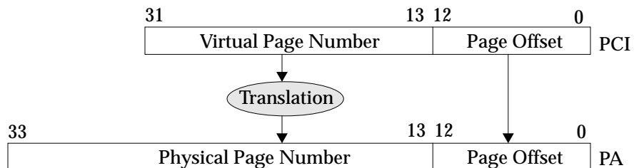
FIGURE 10-4 Virtual to Physical Address Translation for 8K Page Size
