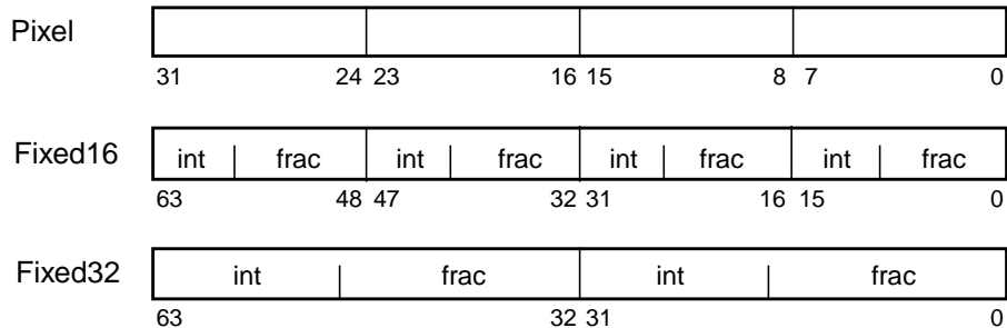
FIGURE 13-1 Graphics Fixed Data Formats
