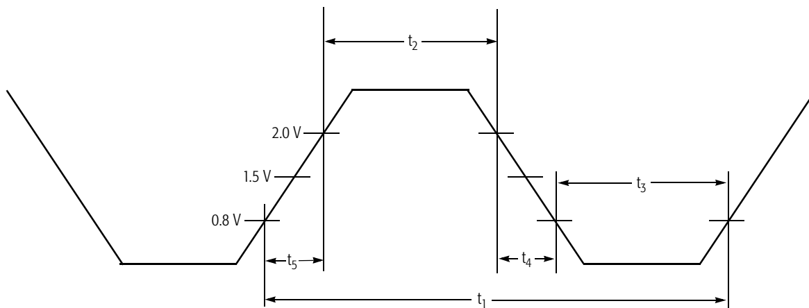
Figure 95. CLK Waveform
