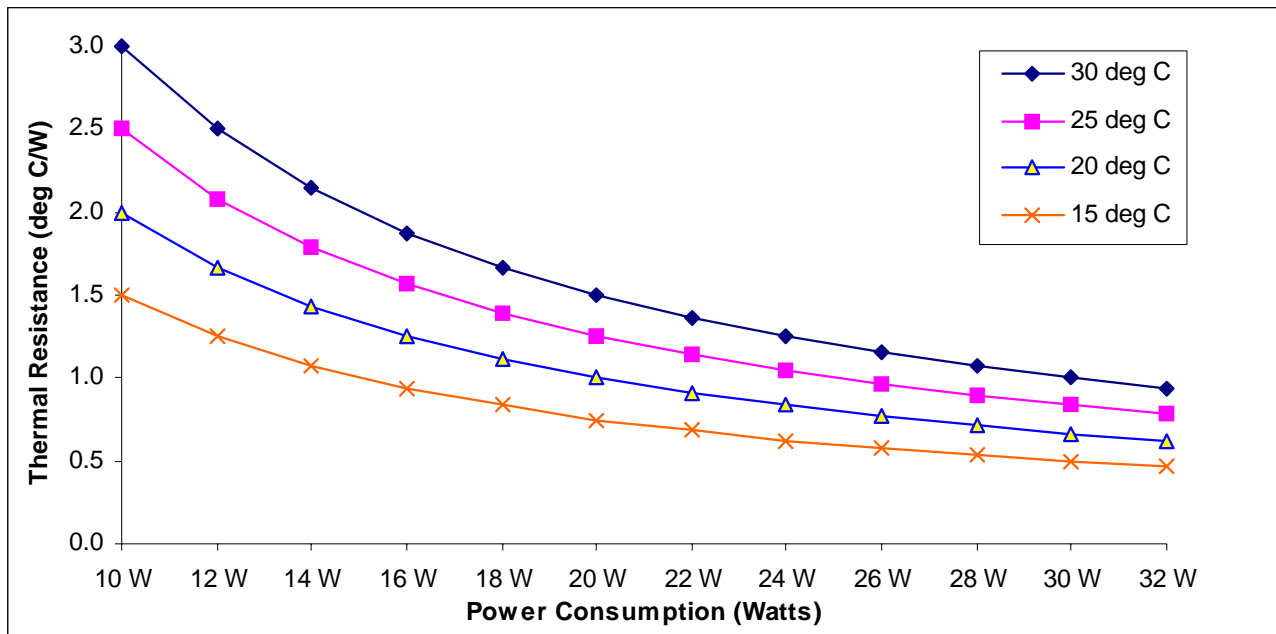
Figure 105. Power Consumption vs. Thermal Resistance
