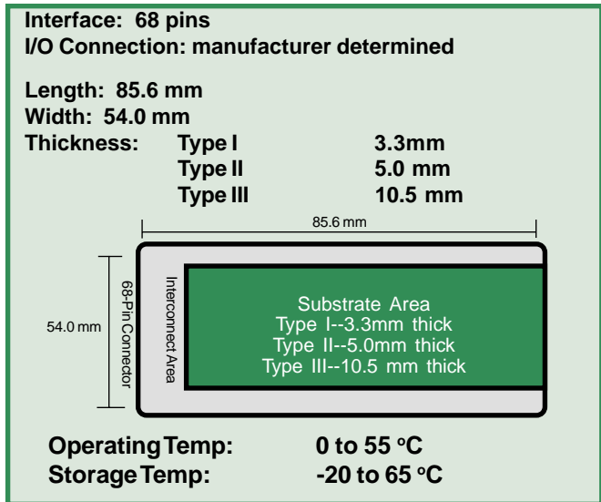
(PCMCIA Card Physical Characteristics)
