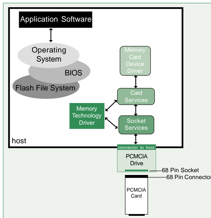
(Block Diagram of a Basic PCMCIA Expansion System)
