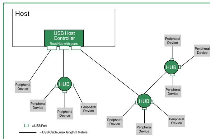
(A Typical USB System)
